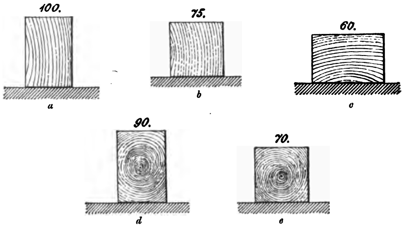
Fig. 43.—Ratios of the strength of different beams of the same section in area, but of different shapes.
